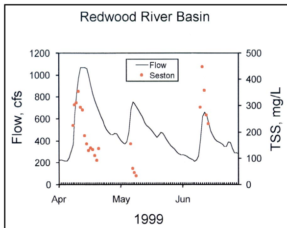
Figure 2. Variations in flow and total suspended sediment concentrations for the period April through June
