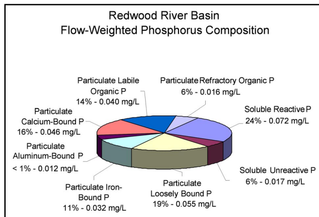
Figure 6. Flow-weight phosphorus composition for the period April through June 1999
