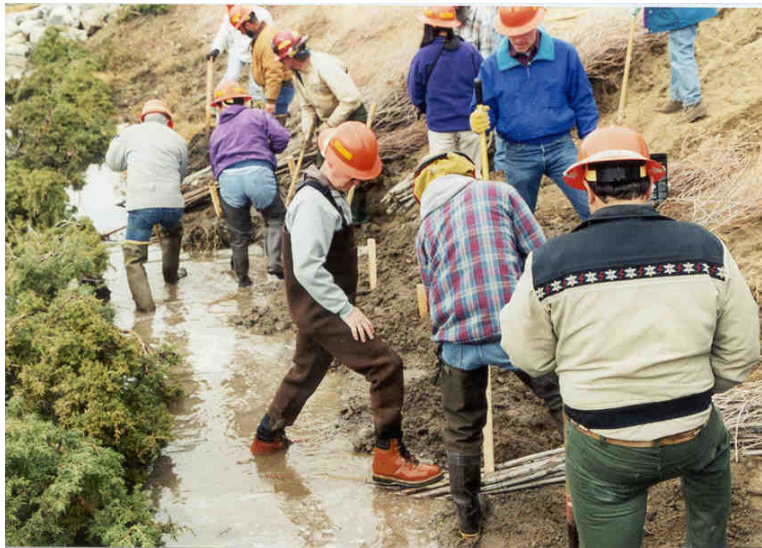
Figure 5. Installation of vertical willow bundles landward of juniper tree revetment; the tree revetment served as toe protection between two barbs and promoted sediment deposition
