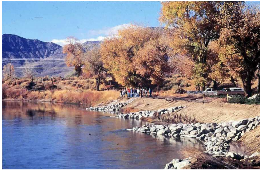
Figure 3. Bioengineering treatments between rock barbs; the barbs are used to deflect currents away from bank (move the thalweg)
