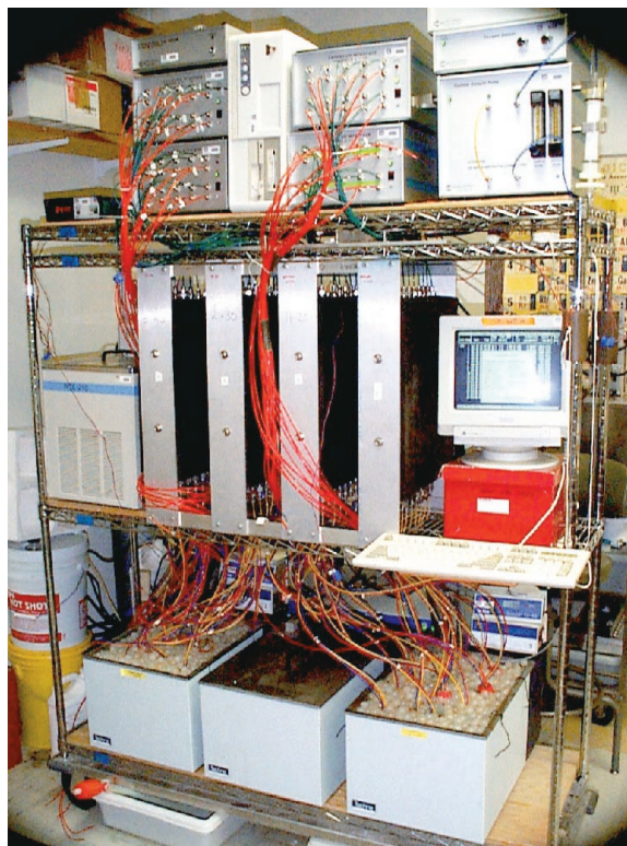
Figure 5. CRREL's temperature-controlled respirometer
