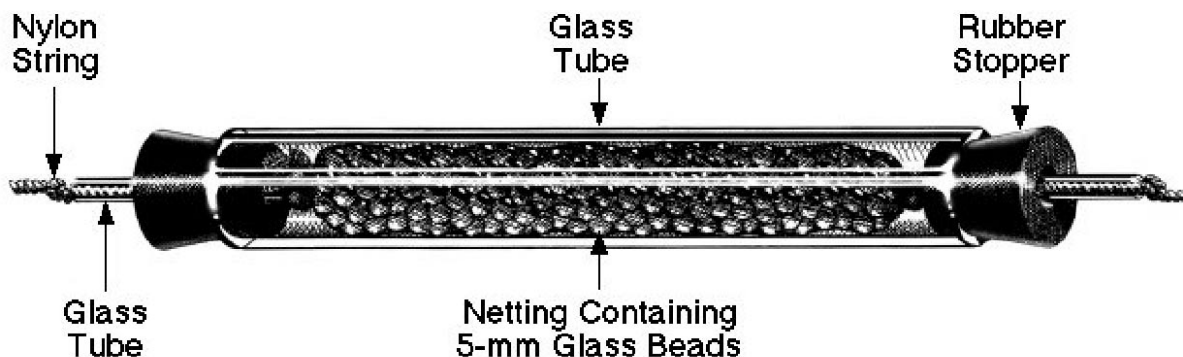
Figure 3. Flow-through sampler designed to collect microbial samples. Rubber stoppers are pulled back when submersed to allow flow through and permit deposition on the surface provided by the glass beads
