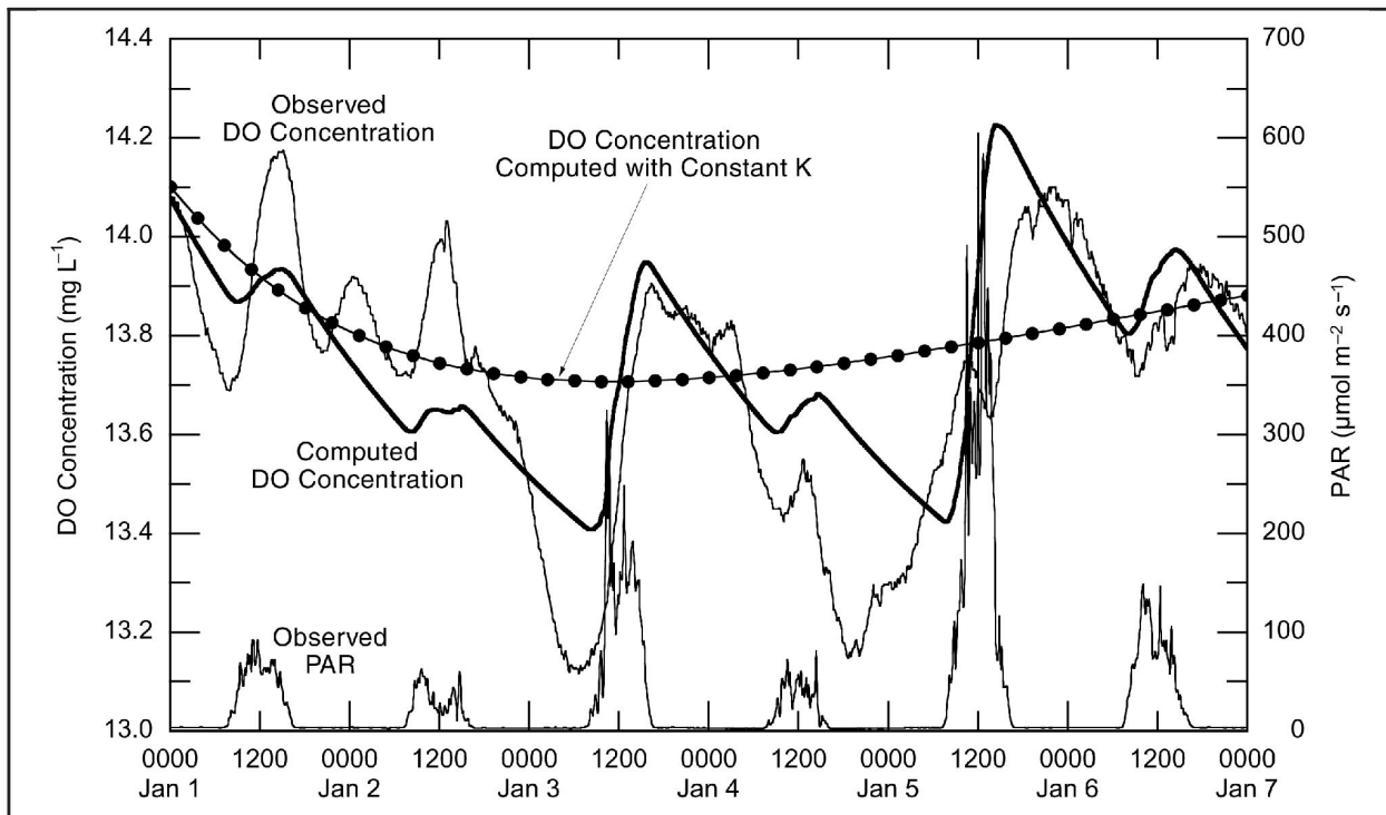
Figure 13. Observed versus computed DO for the open-water period 1-6 January 2000. For comparison, DO computed using constant K_r = 0.5 \text{ d}^{-1} is also shown. Observed PAR is shown for the same period
