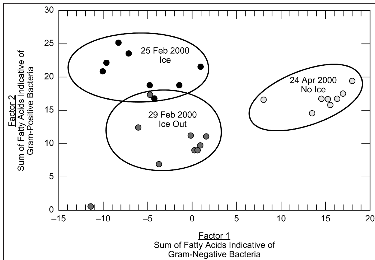
Figure 12. Results of the principal component analysis of fatty acid data obtained from culturable microorganisms collected by the glass bead samplers during the ice-covered period, immediately after ice cover breakup, and well after ice cover breakup
