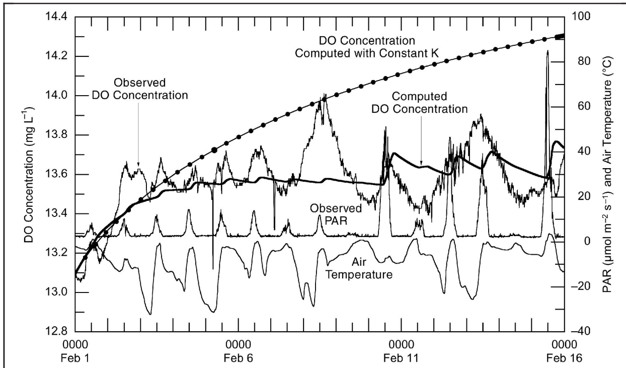
Figure 14. Observed versus computed DO and observed PAR and air temperature during the late ice-covered period 1-15 February 2000. For comparison, DO computed using constant K_r = 0.7 \text{ d}^{-1} is also shown
