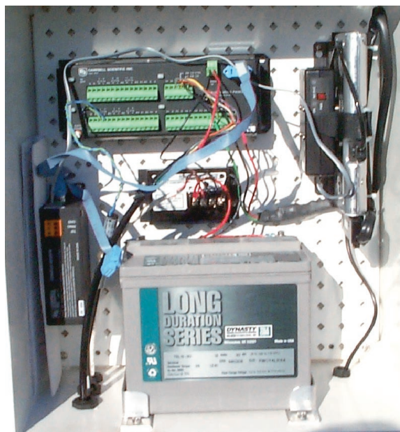
Figure 2. Data acquisition system showing (clockwise from top) Campbell CR10X, cell phone, battery, and modem, with voltage regulator in the center
