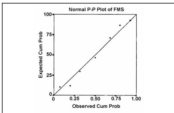
Figure 5. Normal probability plot of fixed monitor station data. (Straight line plots the normal distribution; square symbols are the observed data.)
