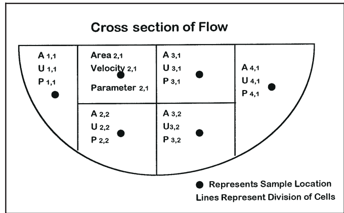
Figure 3. Hypothetical sample scheme for flow-weighting data
