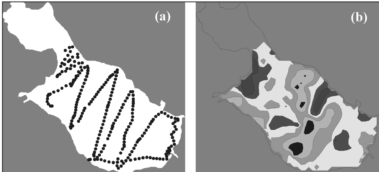
Figure 3. Maps of Laguna San Jose, Puerto Rico, showing the sampling track (a) and the resulting map of surface chlorophyll distribution (b). This demonstrates the real spatial variation possible for even relatively small aquatic systems
