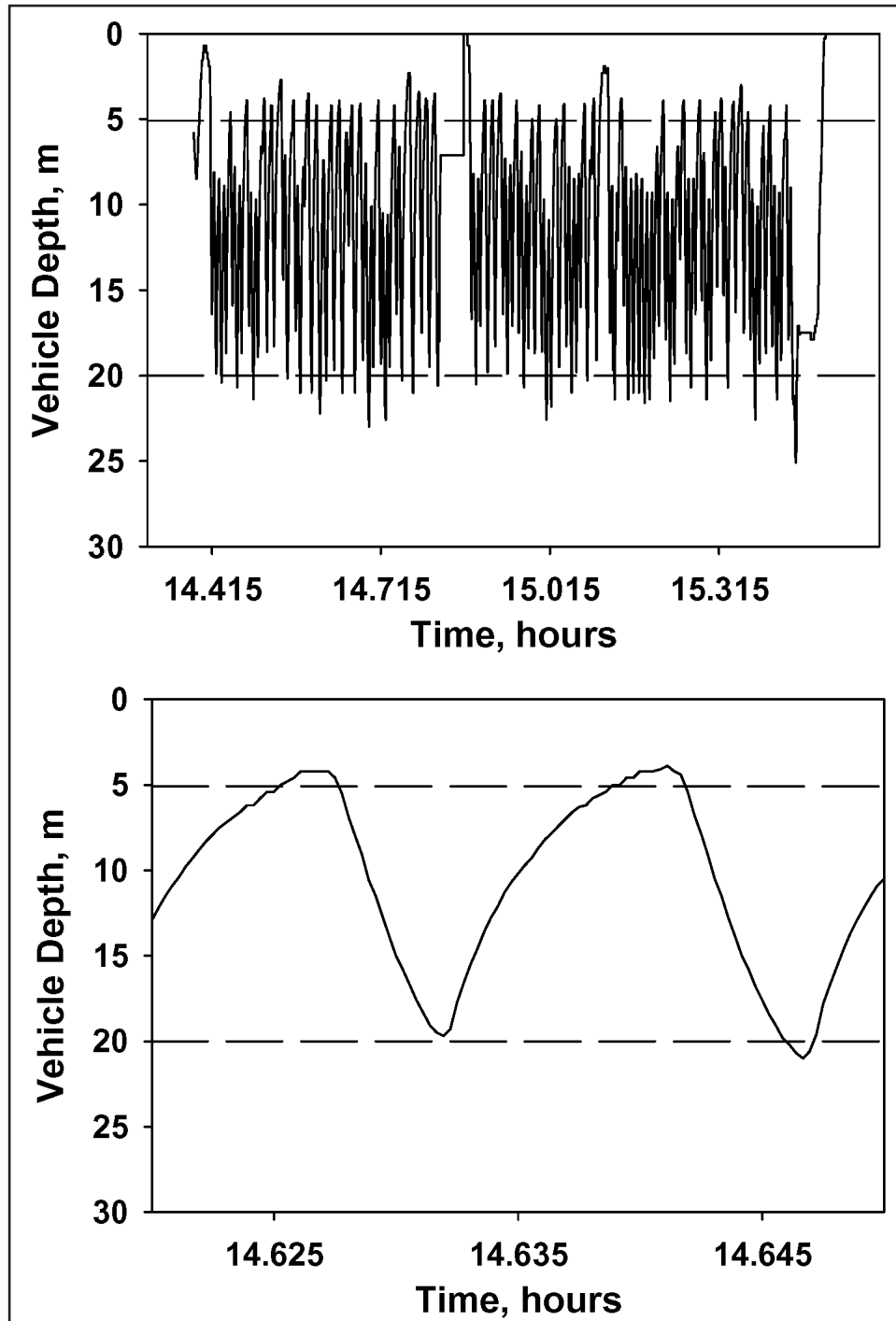
Figure 7. Changes in vehicle depth during a 1-hr deployment of the MiniBAT@n J. Strom Thurmond Lake (upper). Changes in vehicle depth are also displayed on an expanded scale (lower) during two cycles of ascent and descent. Ascending and descending rates averaged 0.53 m/sec and 0.92 m/sec, respectively
