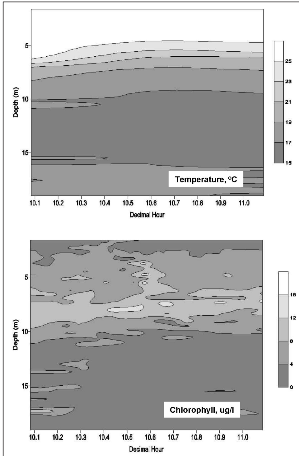
Figure 10. Depth distribution of temperature and chlorophyll concentration along a longitudinal transect in the downstream reach of Richard B. Russell Lake
